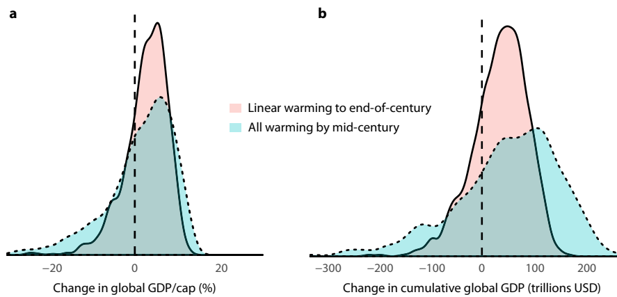
Extended Data Fig. 5 | Robustness under alternative warming paths. Benefit—in terms of per capita GDP (a) and cumulative GDP (b)—of 1.5°C versus 2°C by end of century under the baseline assumption that overall projected warming occurs linearly between the baseline year and 2099 (pink), versus projected benefit assuming that all projected warming occurs by 2049 and temperatures remain constant thereafter (blue). Both
