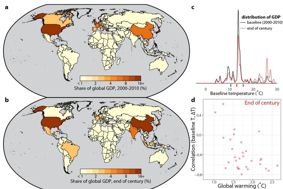
Extended Data Fig. 2 | Global GDP impacts can be negative at +1 °C but positive at +2 °C for some high-temperature-optimum bootstrap runs. a, b, Country share of global GDP at baseline ( a ) and by the end of the century ( b ) under SSP1, assuming no climate change. c, Distribution of global GDP by temperature, under baseline (black) and the end of the century SSP1 without climate change (red dashed); absent climate change, a substantial portion of global GDP is projected to be produced in countries with hotter average temperatures. d, Climate-model-predicted average global warming under RCP2.6 by the end of the century ( x axis) versus the correlation between country-level baseline average temperature and country-level predicted warming in each model. In models that warm less at the global scale, countries that are currently warm tend to exhibit relatively larger warming, while in models that warm more at the global scale, countries that are currently cool tend to exhibit relatively larger warming. Future impacts on global GDP are a sum of country-specific impacts, which are a function of where each country is on the temperature
