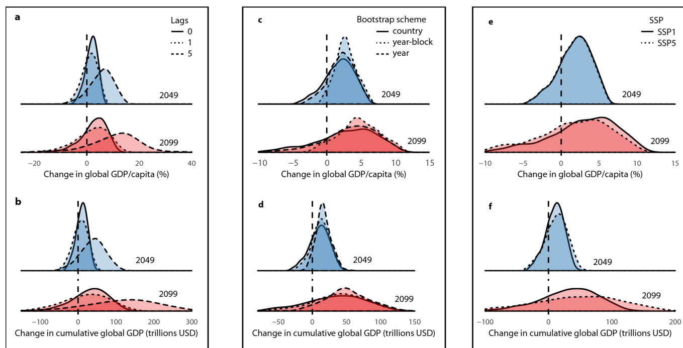
Extended Data Fig. 4 | Robustness of results to alternative specifications. Change in global GDP per capita in 2049 and 2099 based on regression models that include 0, 1 or 5 lags ( a and b ); bootstrap schemes that sample by country, five-year block or single year ( c and d ); or
